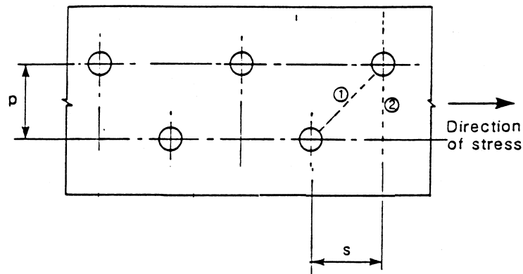
Figure 6.1: Staggered holes
