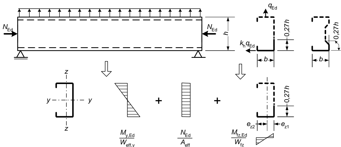
Figure 10.2: Superposition of stresses ((Figure to be modified: 0,27h to be replaced by 1/5h resp. 1/6h))
