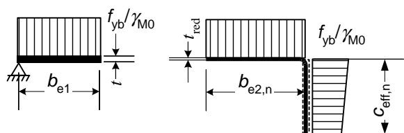
Figure 5.10: Compression resistance of a flange with an edge stiffener
