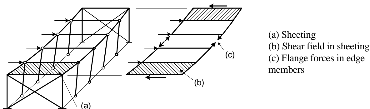
Figure 10.12: Stressed skin action in a flat-roof building
