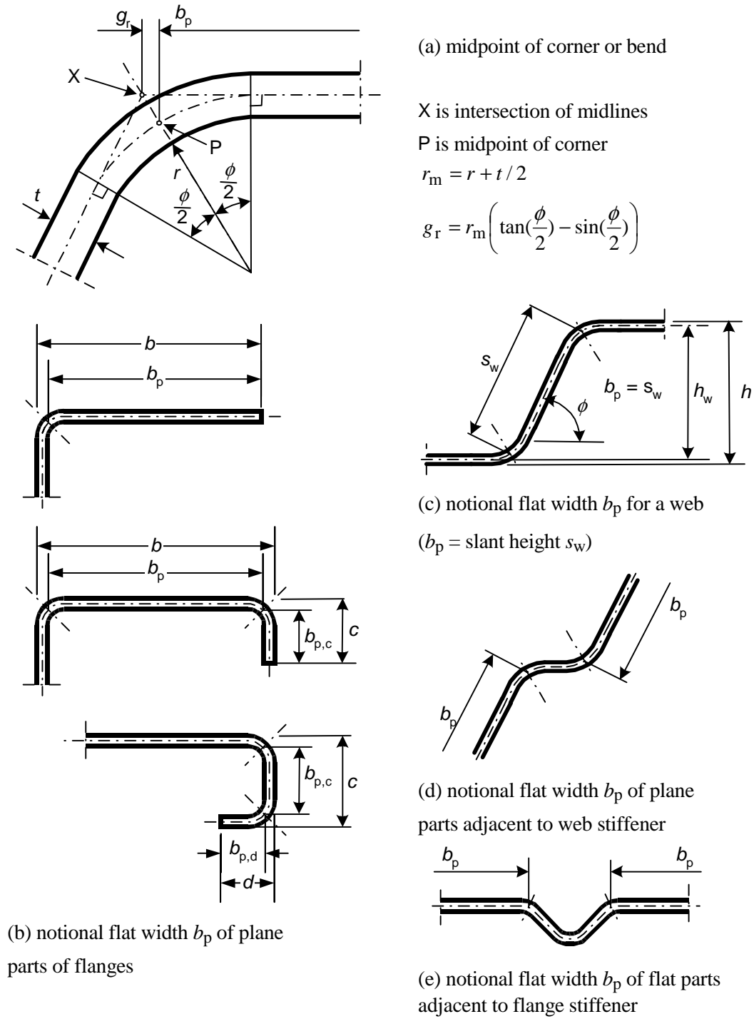
Figure 5.3: Notional widths of plane cross section parts b_p allowing for corner radii
