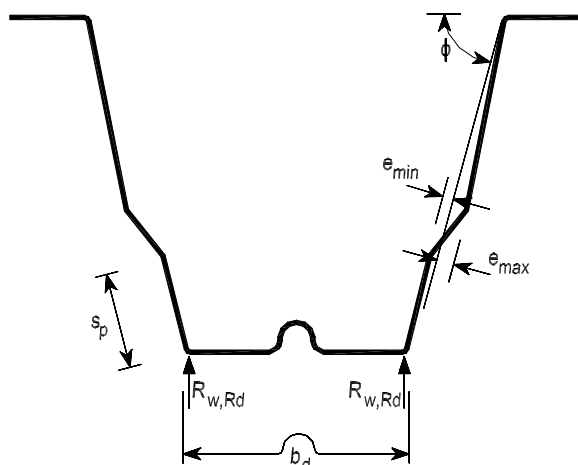
Figure 6.10: Stiffened webs
