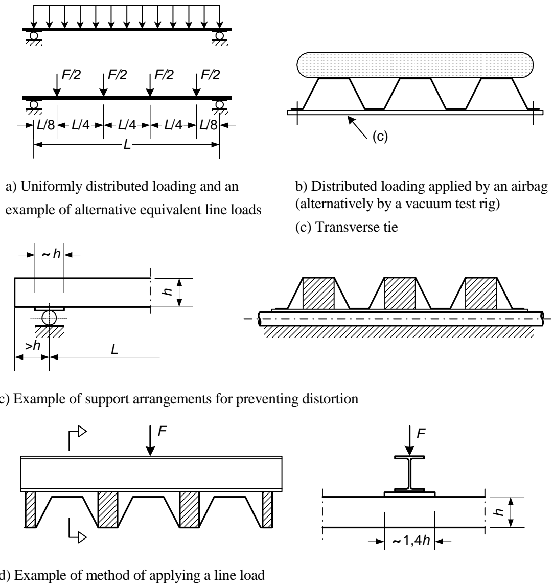
Figure A.2: Test set-up for single span tests
