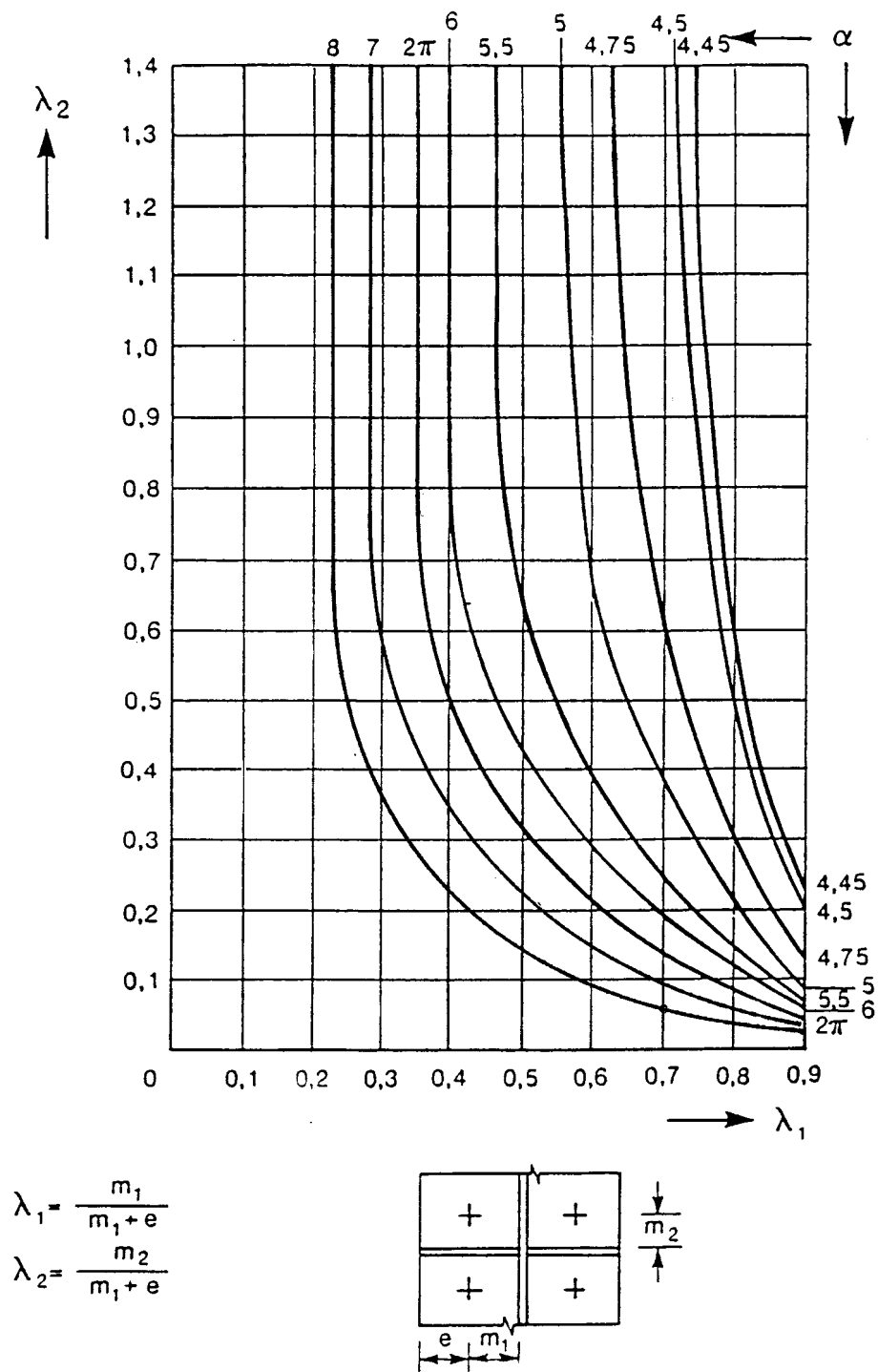
Figure 6.12: Values of \alpha for stiffened column flanges and end-plates
