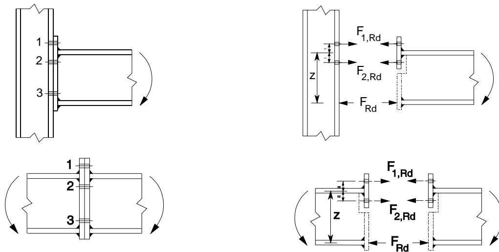
Figure 6.17: Simplified models for bolted joints with extended end-plates
