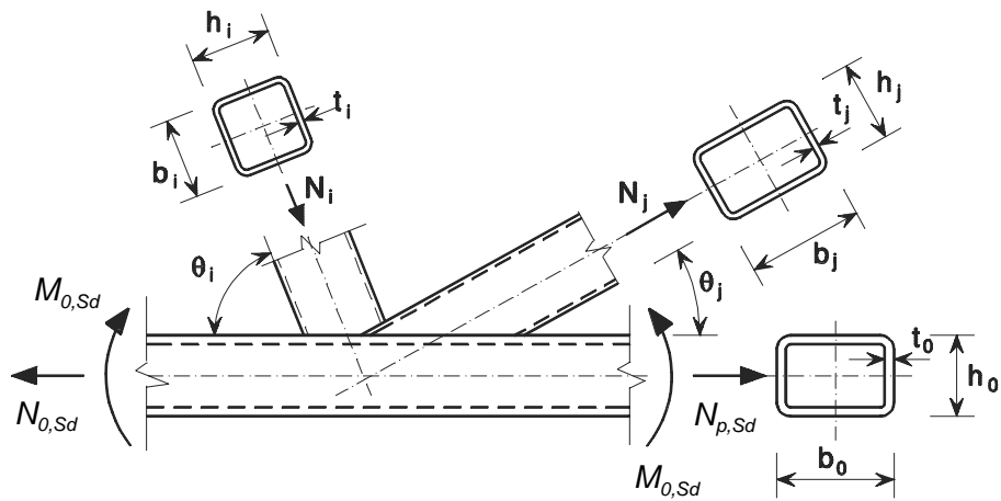
c) Overlap joint with two brace members
