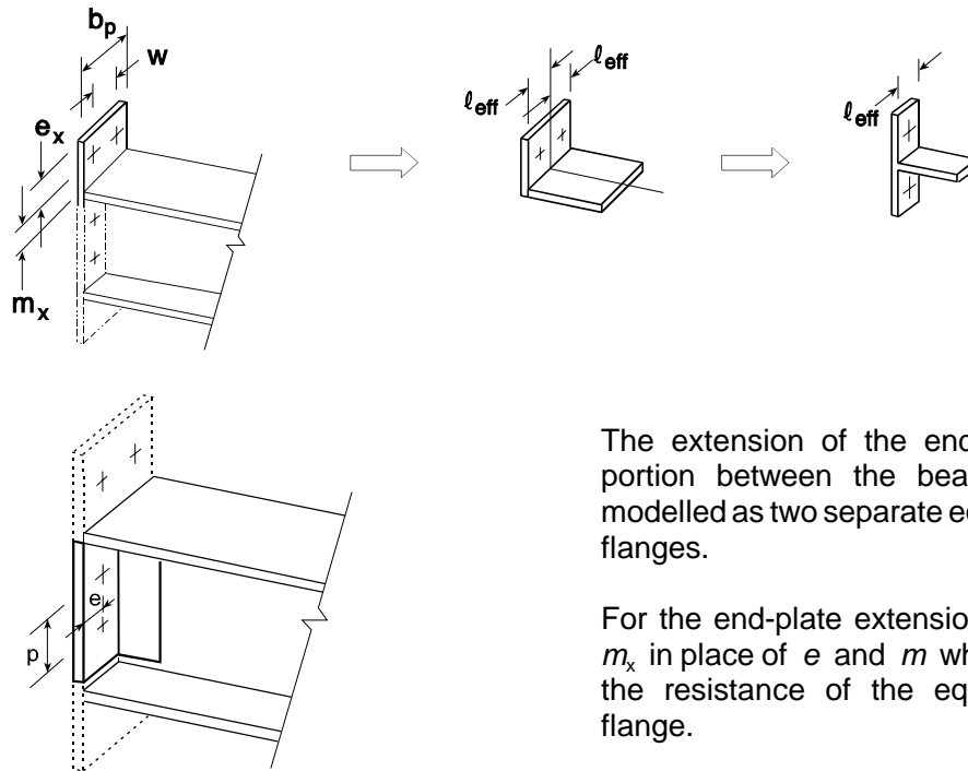
Figure 6.11: Modelling an extended end-plate as separate T-stubs
