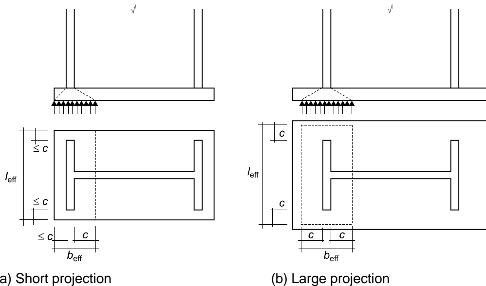
Figure 6.5: Area of equivalent T-Stub in compression
