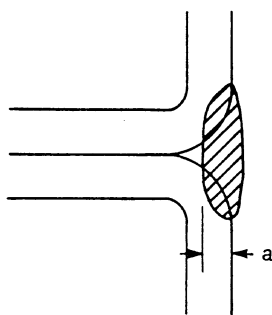
Figure 7.5: Effective throat of flare groove welds in rectangular structural hollow section
