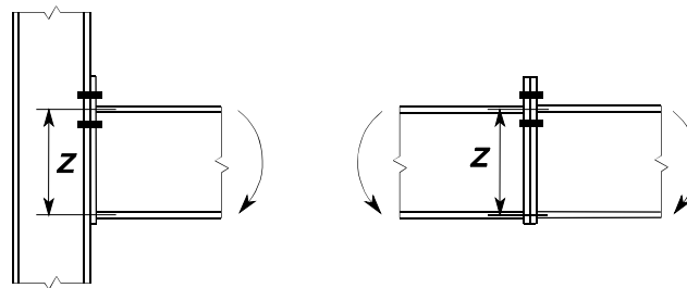
Figure 6.21: Lever arm z for simplified method
