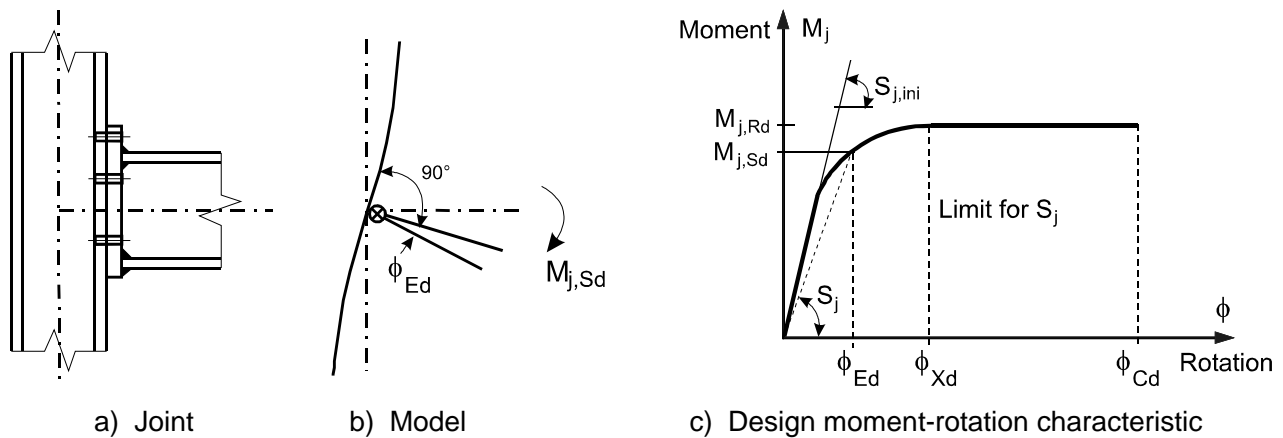
Figure 6.1: Design moment-rotation characteristic for a joint
