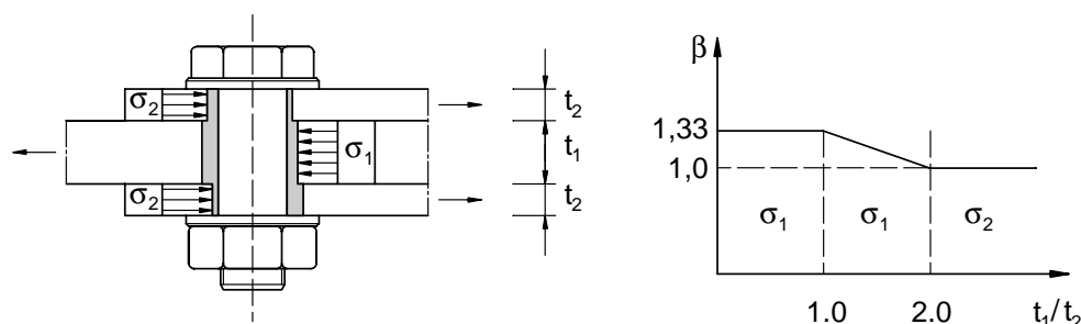
Figure 3.6: Increase of f_{b,resin} by a factor \beta in case of thick cover plates
