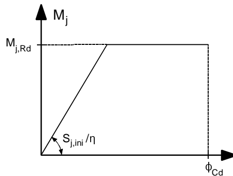
Figure 5.2: Simplified bi-linear design moment-rotation characteristic
