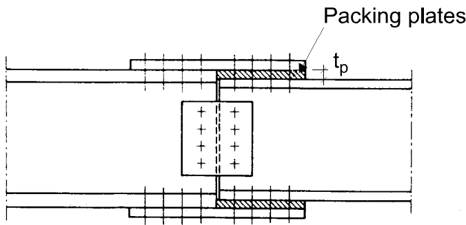
Figure 3.5: Fasteners through packings
