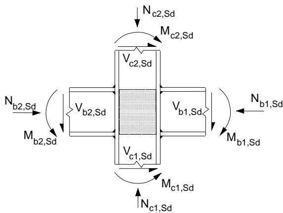
a) Values at periphery of web panel.
