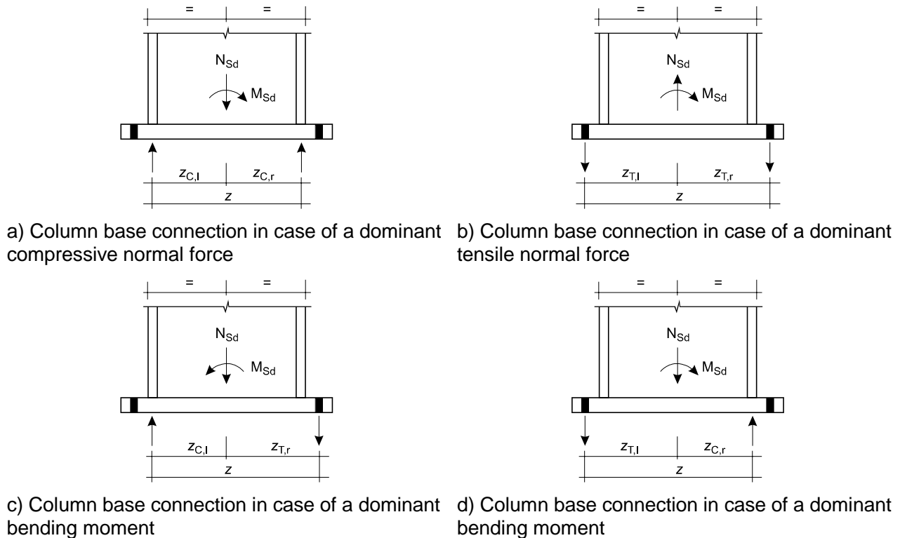
Figure 6.19: Determination of the lever arm z for column base connections
