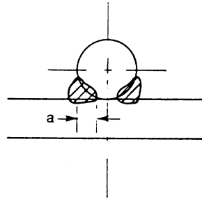
Figure 4.2: Effective throat of flare groove welds in solid sections
