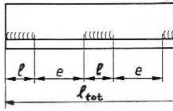
Figure 4.7: Calculation of weld forces for intermittent welds
