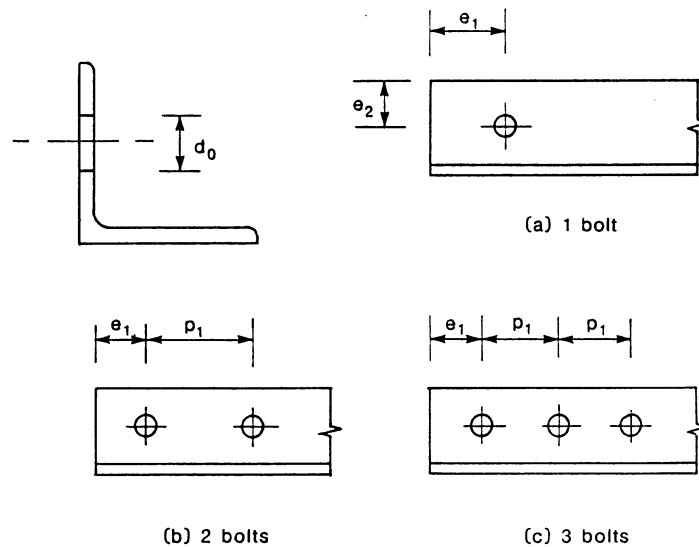
Figure 3.9: Connections of angles
