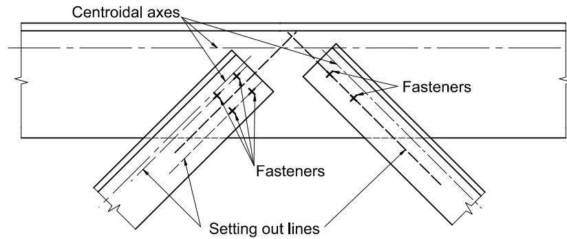
Figure 1.5: Setting out lines
