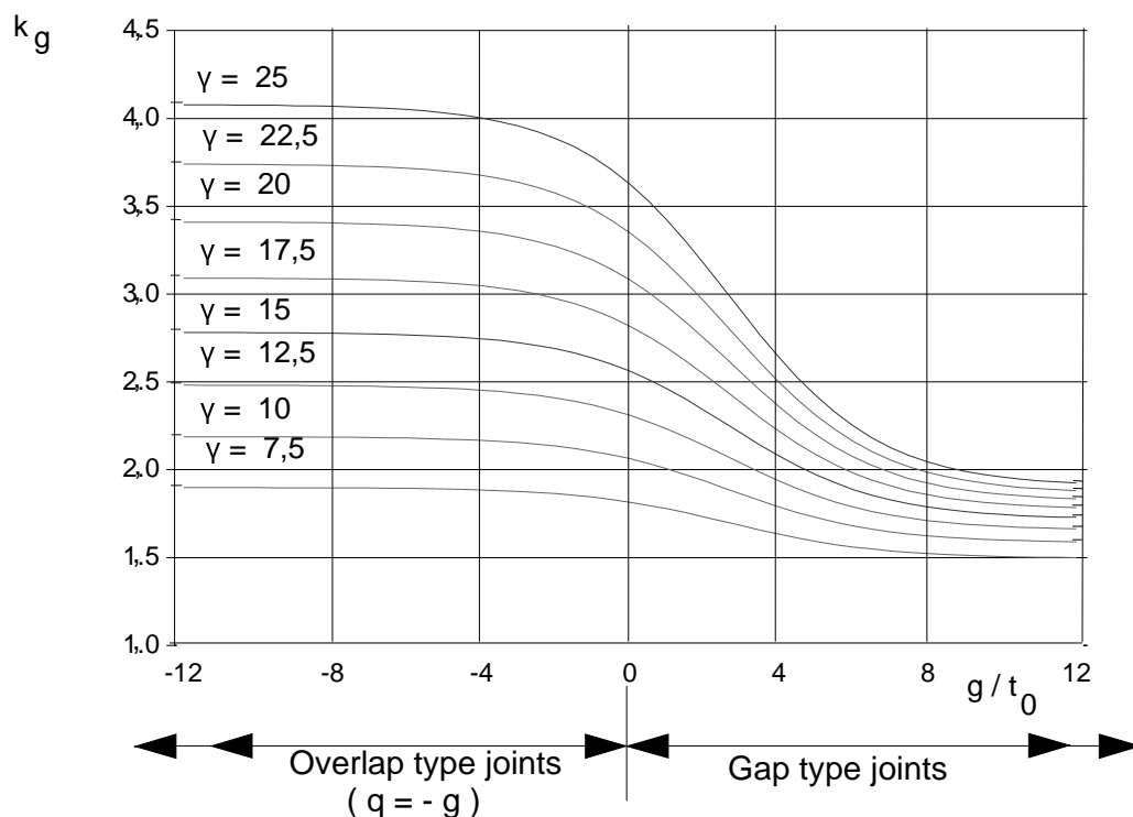
Figure 7.6: Values of the factor k_g for use in table 7.2
