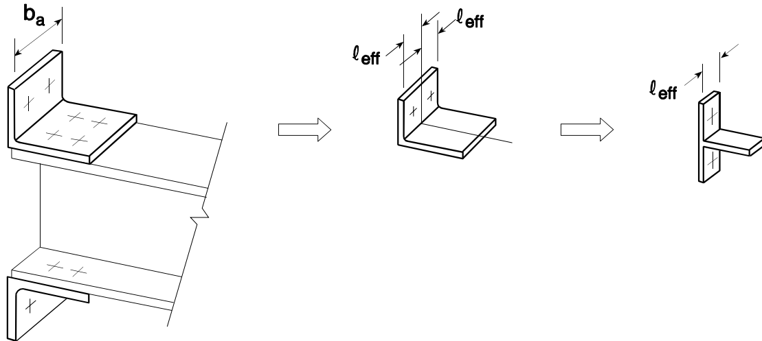
Figure 6.13: Effective length l_{\text{eff}} of an angle flange cleat
