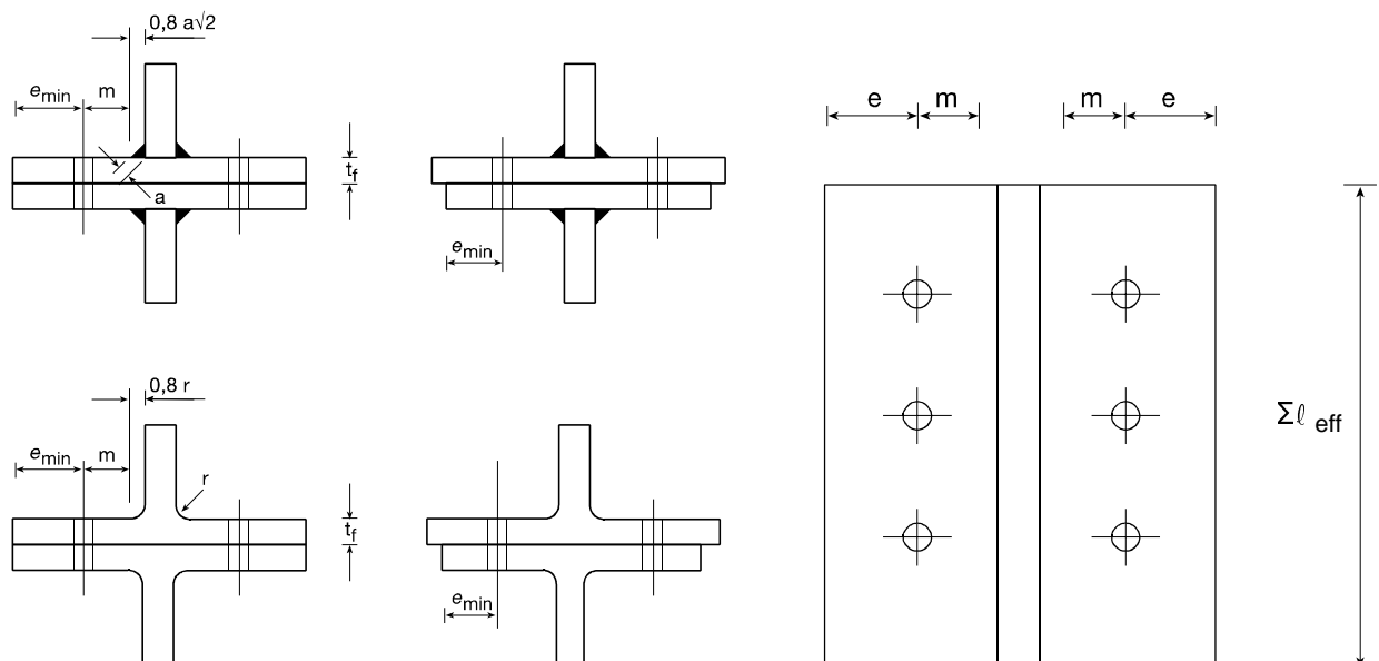
Figure 6.3: Dimensions of an equivalent T-stub flange
