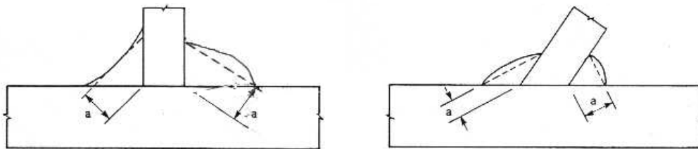
Figure 4.3: Throat thickness of a fillet weld
