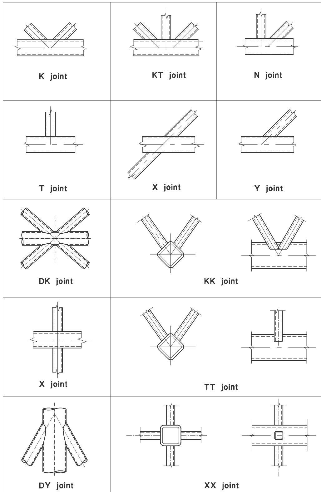
Figure 7.1: Types of joints in hollow section lattice girders
