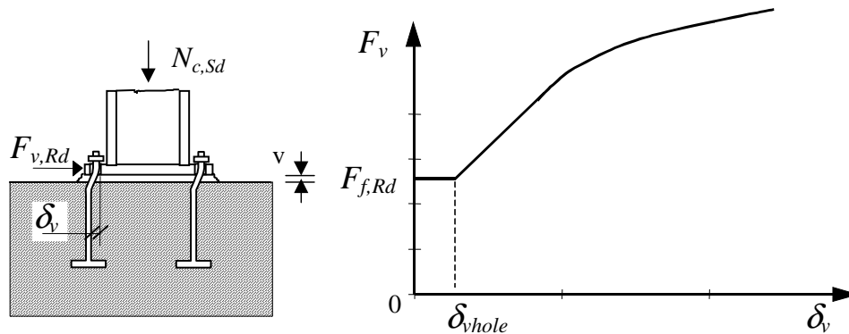
Figure 6.2: Column base loaded by normal force and shear load
