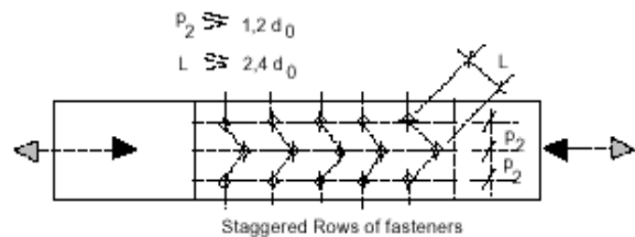
b) Symbols for staggered spacing
