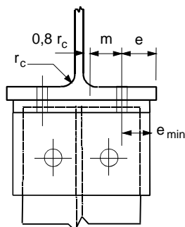
c) Angle flange cleats.
