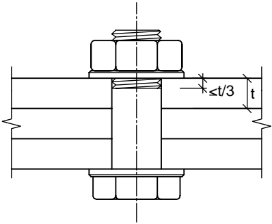
Figure 3.2: Threaded portion of the shank in the bearing length for fit bolts
