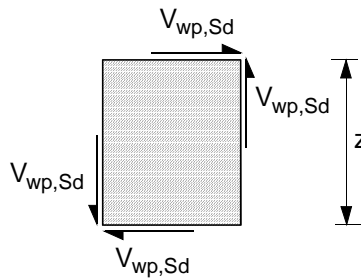
b) Shear forces in web panel.
