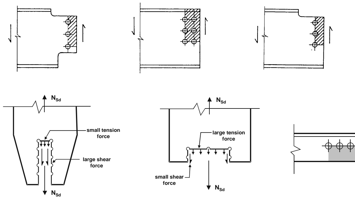
Figure 3.8: Block tearing
