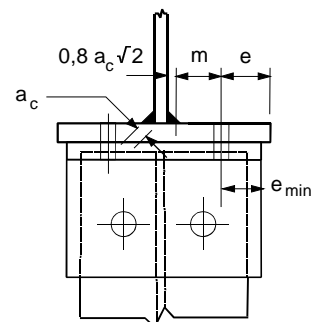
Figure 6.9: Definitions of e , e_{\min} , r_c and m
