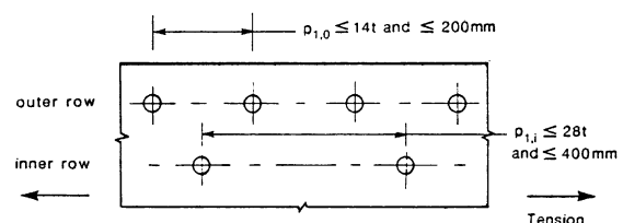
d) Spacing in tension members
