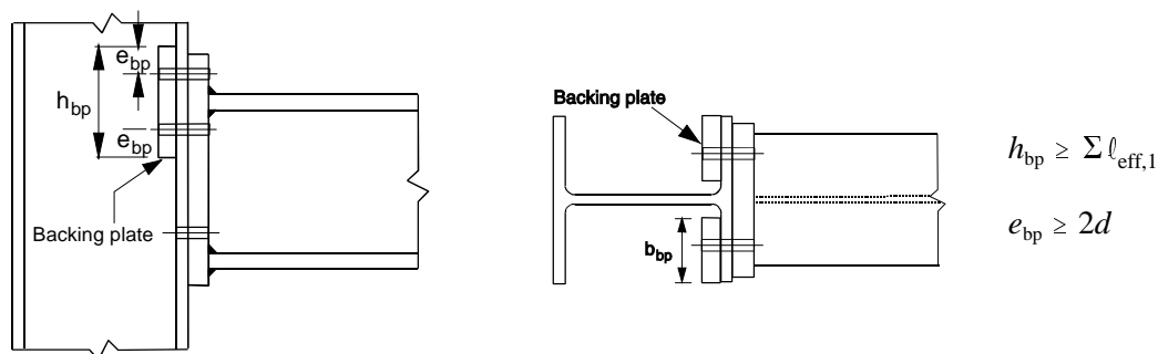
Figure 6.4: Column flange with backing plates
