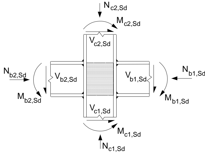
a) Forces and moments acting on joint, at periphery of web panel.
