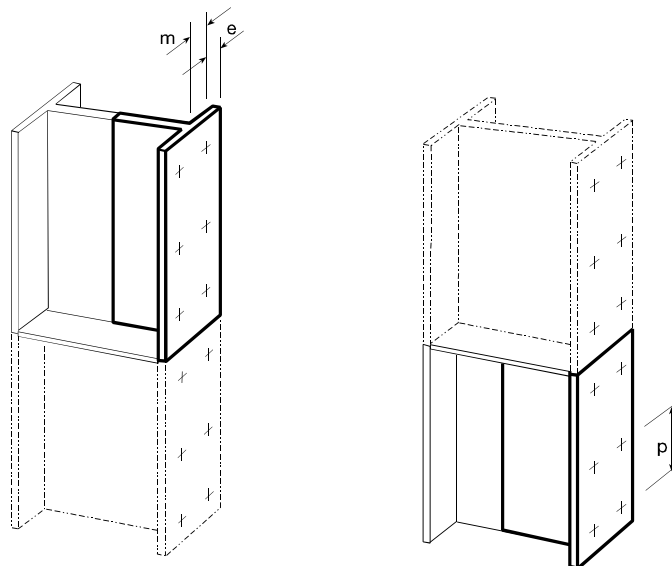
Figure 6.10: Modelling a stiffened column flange as separate T-stubs
