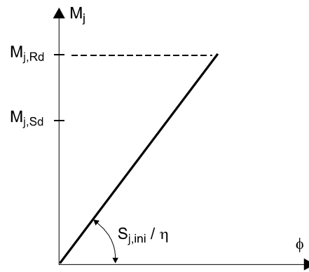
Figure 5.1: Rotational stiffness to be used in elastic global analysis
