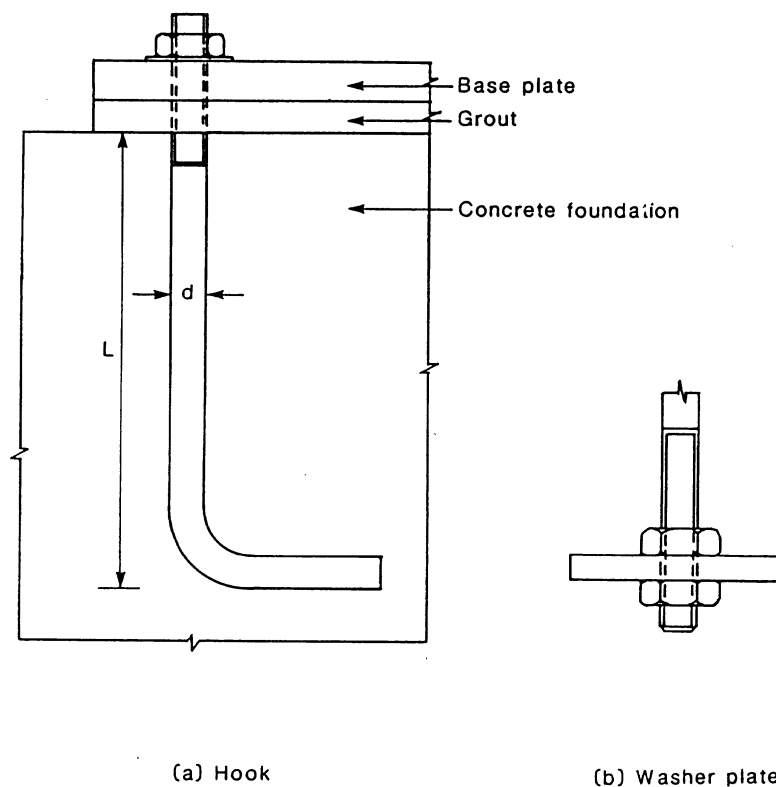
Figure 6.15: Anchorage of anchor bolts
