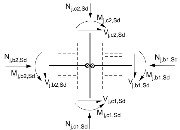
b) Values at intersection of member centrelines.
