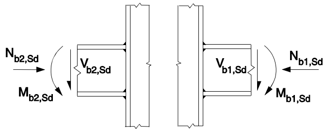
c) Connections, with forces and moments in beams.
