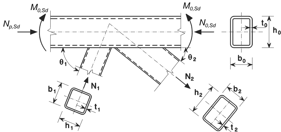
b) Gap joint with two brace members
