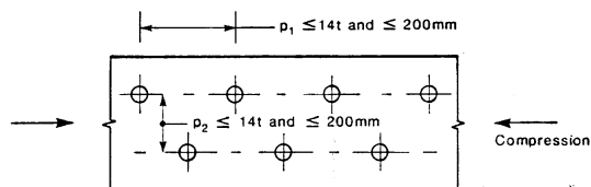
c) Staggered spacing - compression
