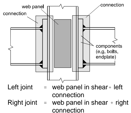
b) Double-sided joint configuration
