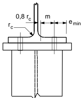
b) Welded end-plate wider than column flange.
