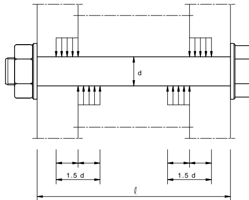
Figure 3.7: Limiting effective length for long injection bolts
