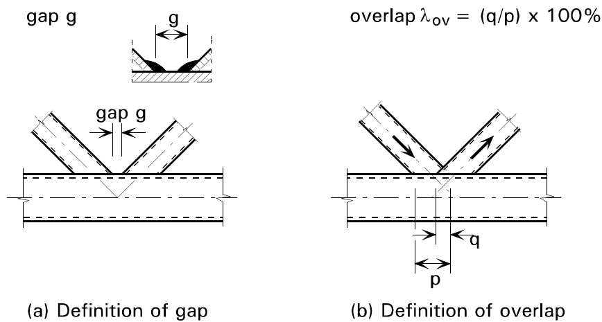
Figure 1.3: Gap and overlap joints.
