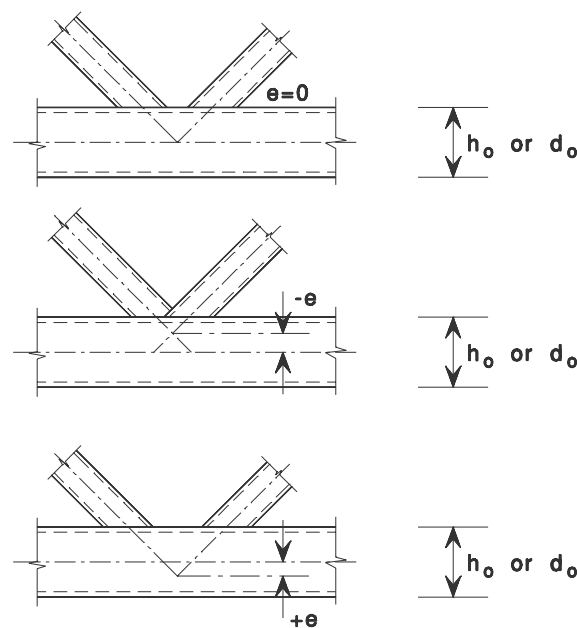
Figure 5.3: Eccentricity of joints.
