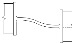
Figure 6.8: 'Column-sway' buckling mode of an unstiffened web
