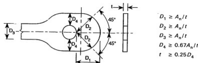
Figure 3.11: Pin-ended tension member
