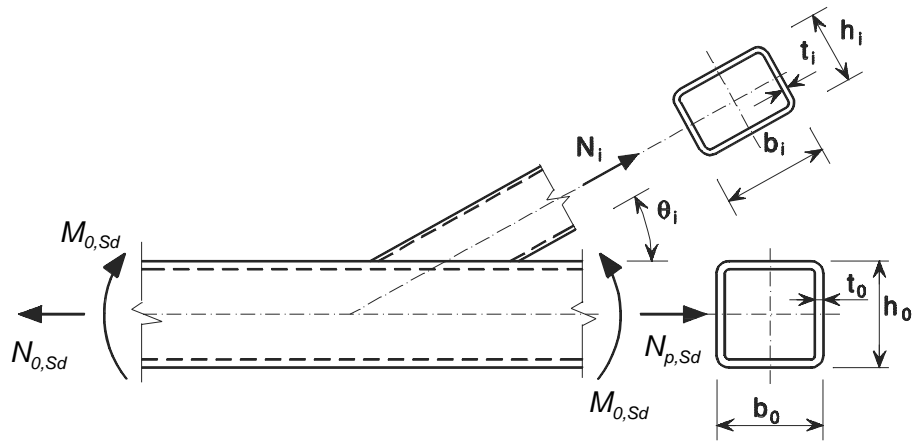
a) Joint with single brace member
