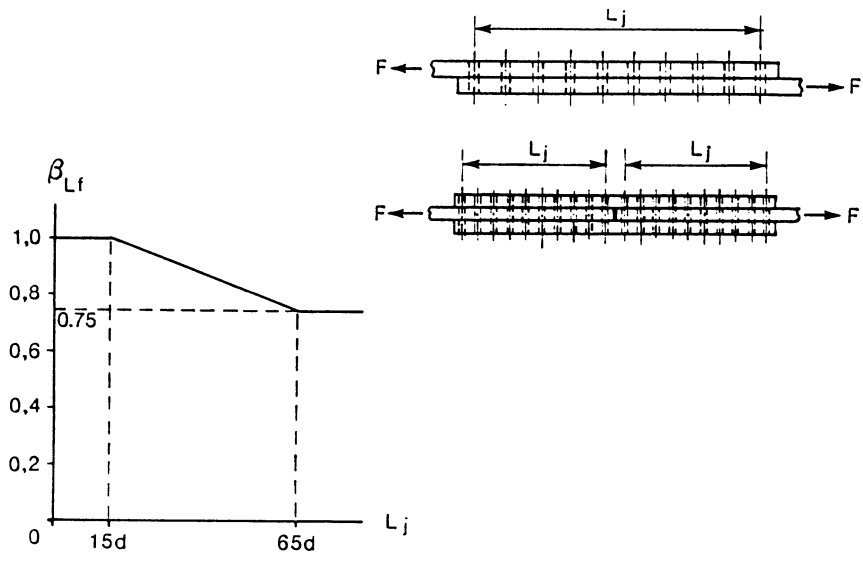
Figure 3.4: Long joints
