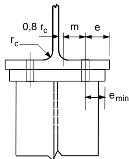
a) Welded end-plate narrower than column flange.
